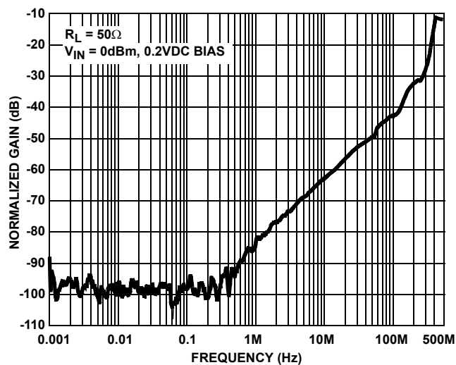
FIGURE 14. OFF-ISOLATION
