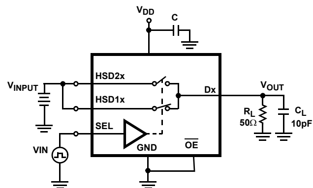
FIGURE 1. SWITCHING TIMES
