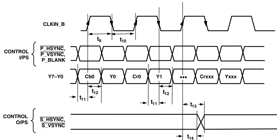
Figure 5. PS 4:2:2 1 x 8-Bit Interleaved @ 27 MHz, Input Mode: PS Input Only (Input Mode at Subaddress 01h = 100)
